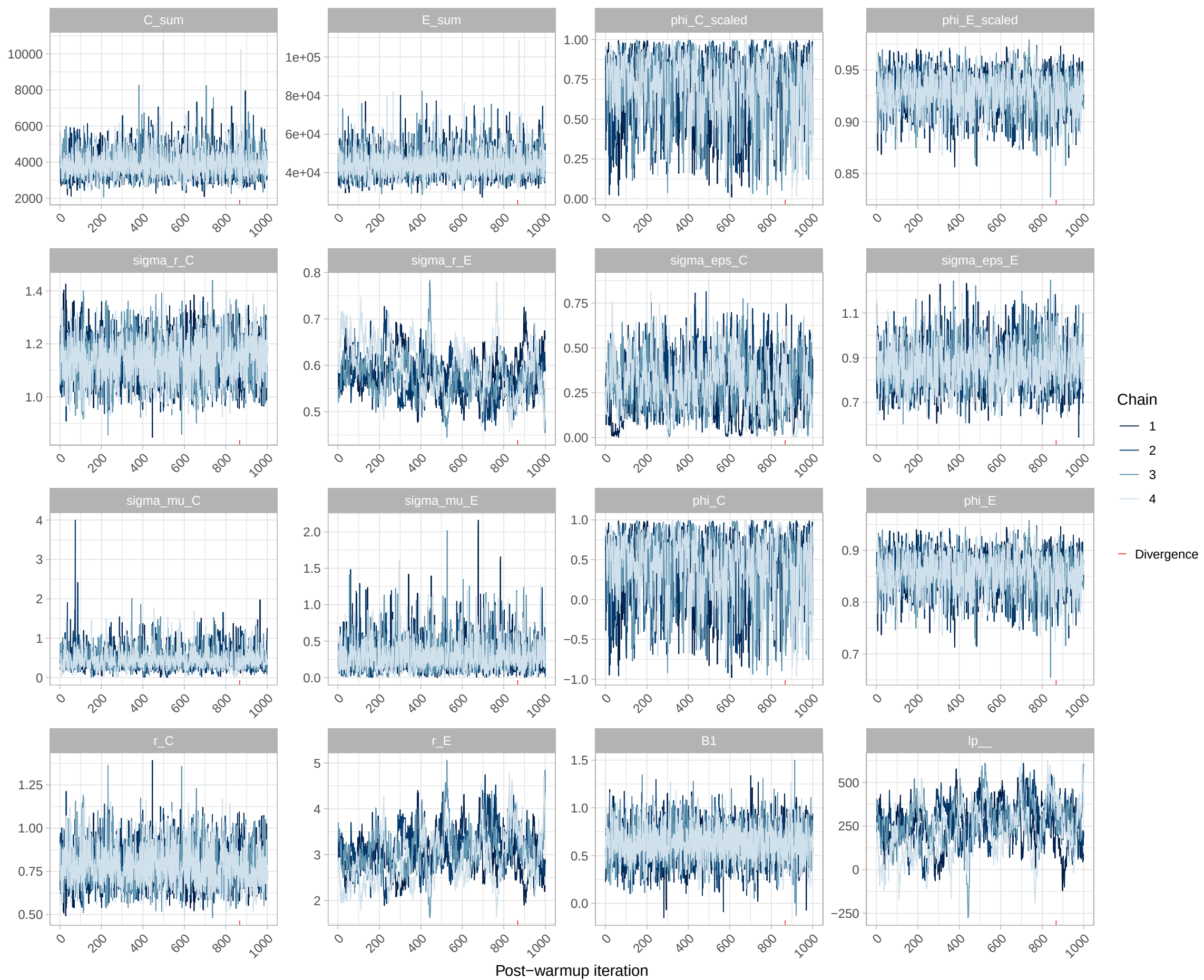
Trace plots for catch group: Steelhead_Adult_UM_Released
